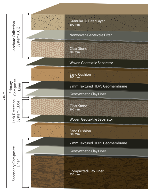
BASE LINER SYSTEM CROSS SECTION
