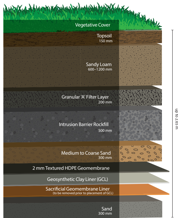
COVER SYSTEM CROSS SECTION
