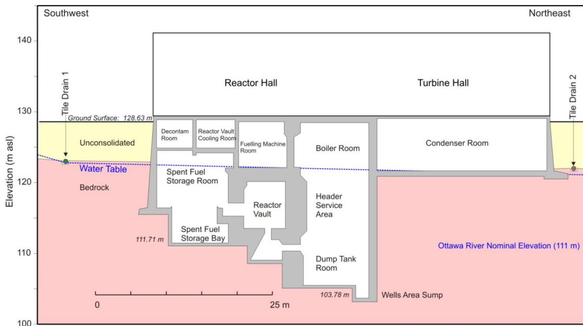
Figure 6-2 Southwest – Northeast cross section through the NPDWF.
